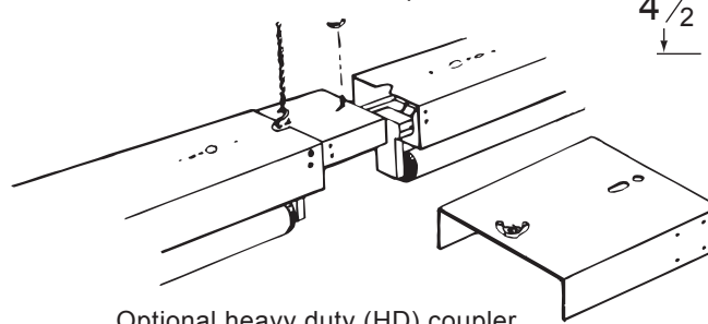
204C Coupler
